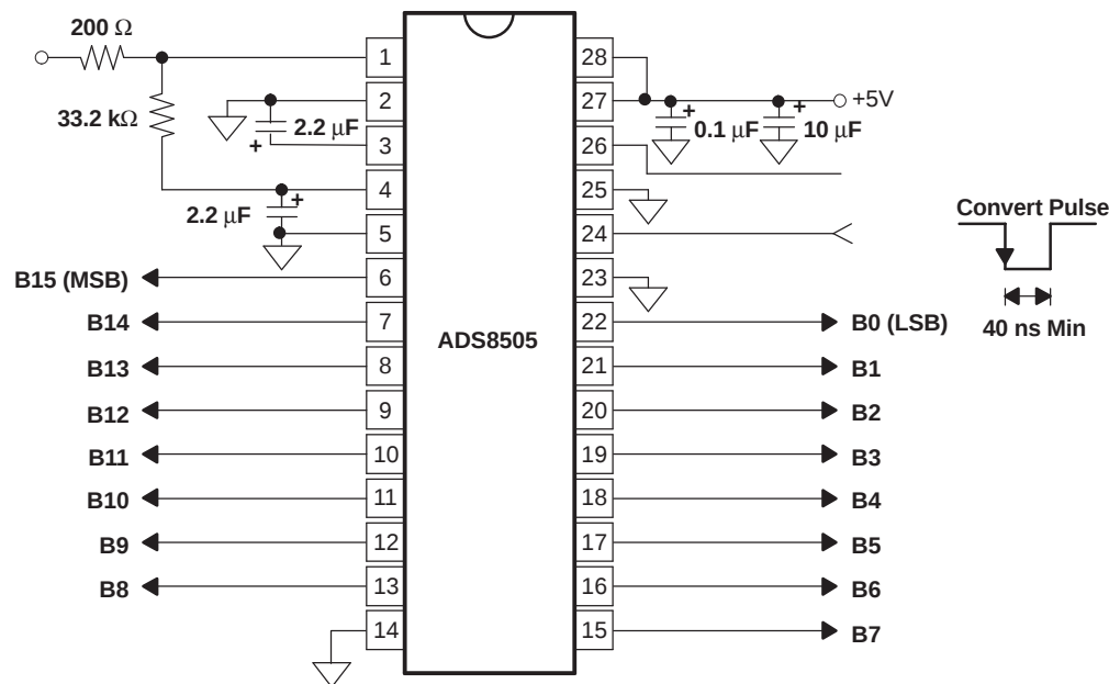
Figure 21. Basic Operation
