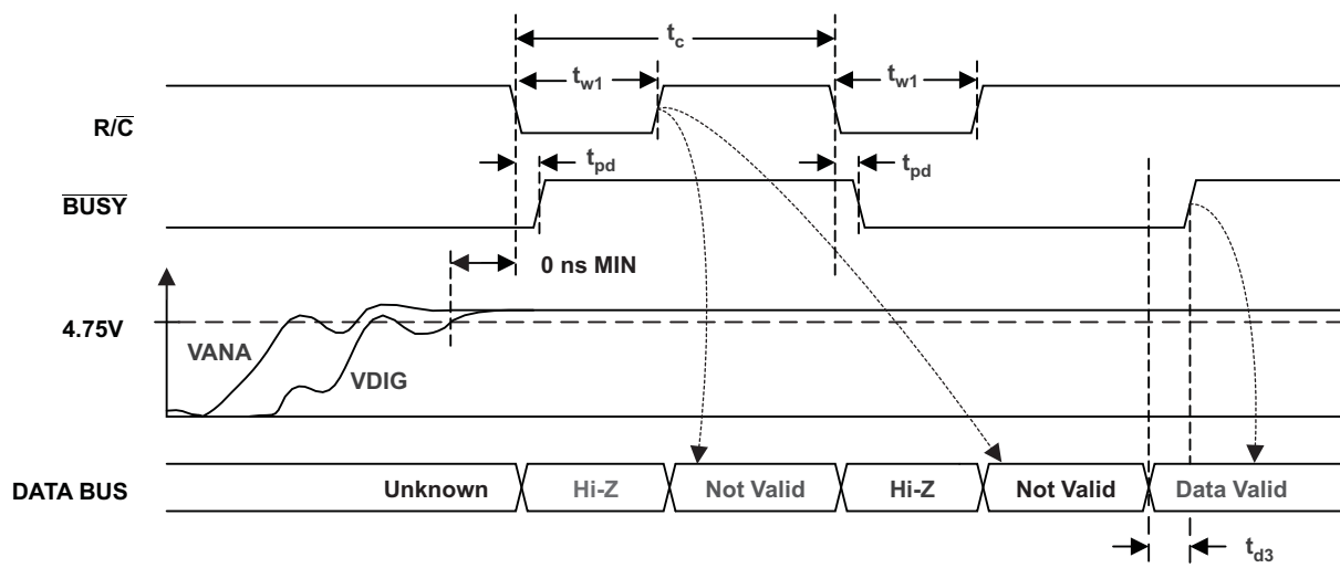
Figure 26. ADC Reset
